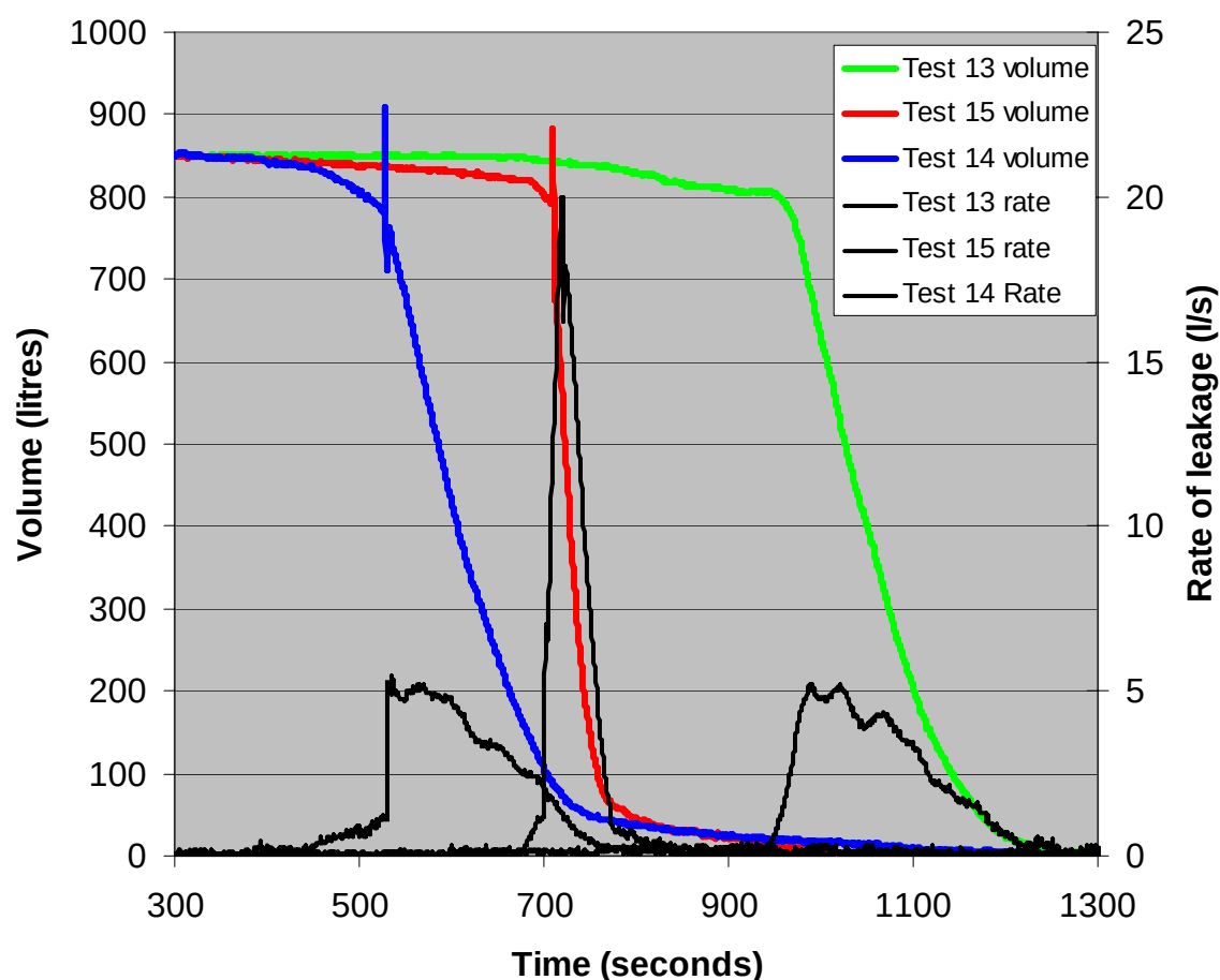
Figure 13: Liquid loss in Tests 13 ,14 and 15
